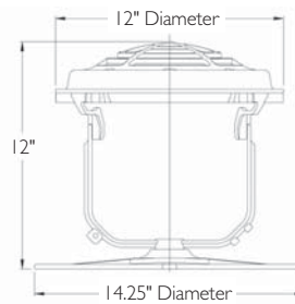
Fountain Fixture for large lights Part No. 560000 (Light sold separately)
